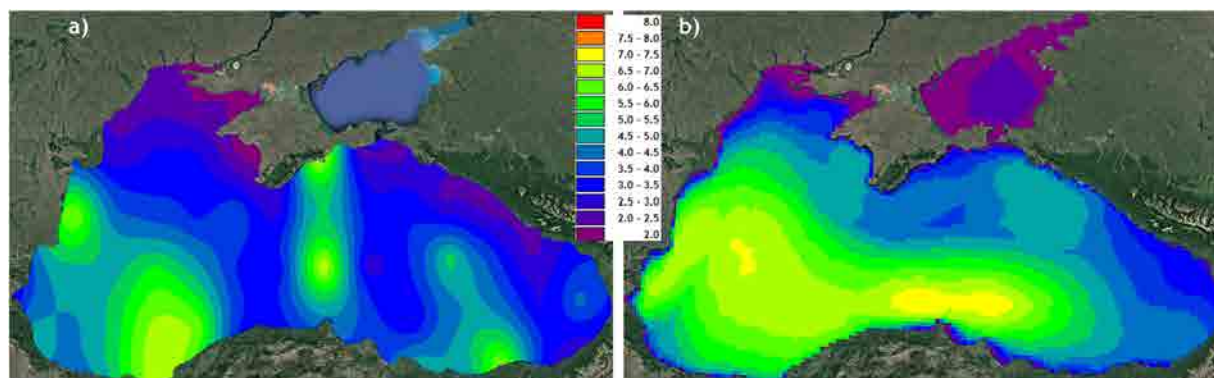
Figure 4 Maximum significant wave heights [m] in the Black Sea in the period from December 1, 2017 to September 30, 2018. (a) Generalization of satellite data; (b) modeling results.
